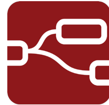
Node-RED
